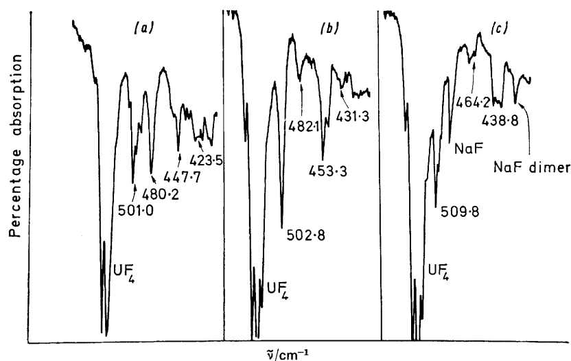
FIGURE 5 Infrared spectra of \text{MF}-\text{UF}_4 systems in argon matrices: \text{M} = \text{Cs} (a), \text{K} (b), and \text{Na} (c)
